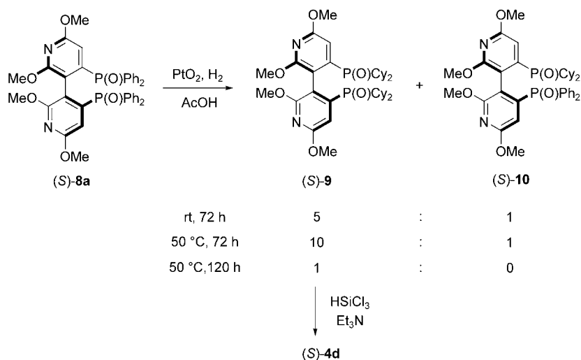
Scheme 4. The synthetic route towards 4d .
