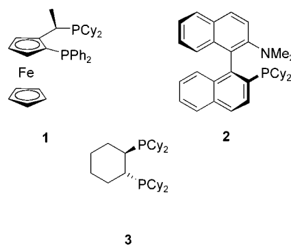
Scheme 1. Some chiral ligands containing dicyclohexylphosphine group.
