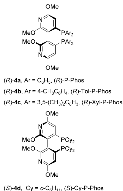
Scheme 2. Chiral dipyridylphosphine ligands 4 .
