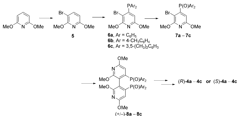
Scheme 3. The synthetic route towards 4a–4c .
